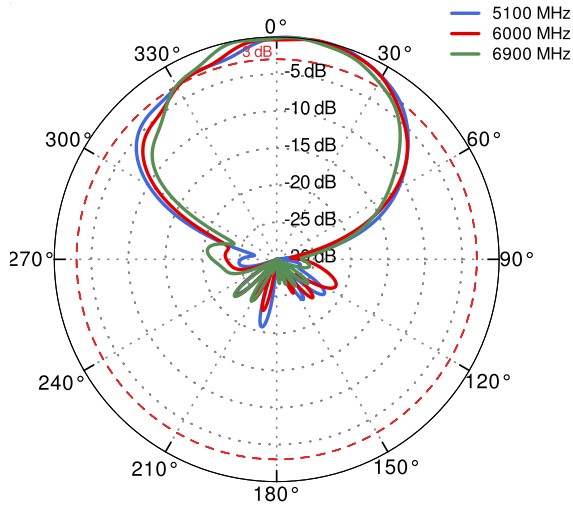
PORT 1&3 ELEVATION
